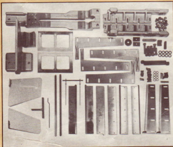
The 4th and 5th Knife Attachment includes: required mounting brackets, set-up gauge, and 2 complete sets of knives (total of 12 knives).
