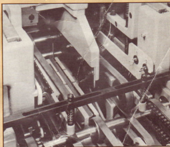
The 4th and 5th Knife mounted on the Model DSS/890 Trimmer for 2-up production.
